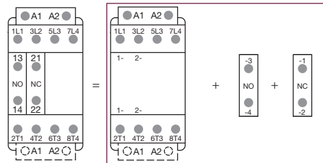
Combination 11 = AF09 ... AF38..-40-00+ CA4-10 + CA4-01
