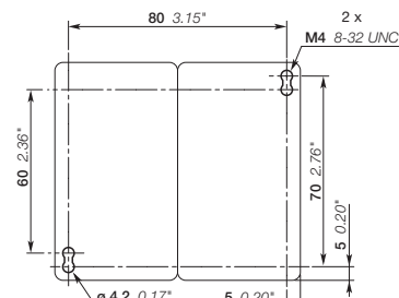
AF26..-40-00, AF38..-40-00 + VEM4 mechanical and electrical interlock set
