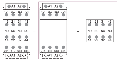
Combination 22 = AF09 ... AF38..-40-00 + CA4-22E
